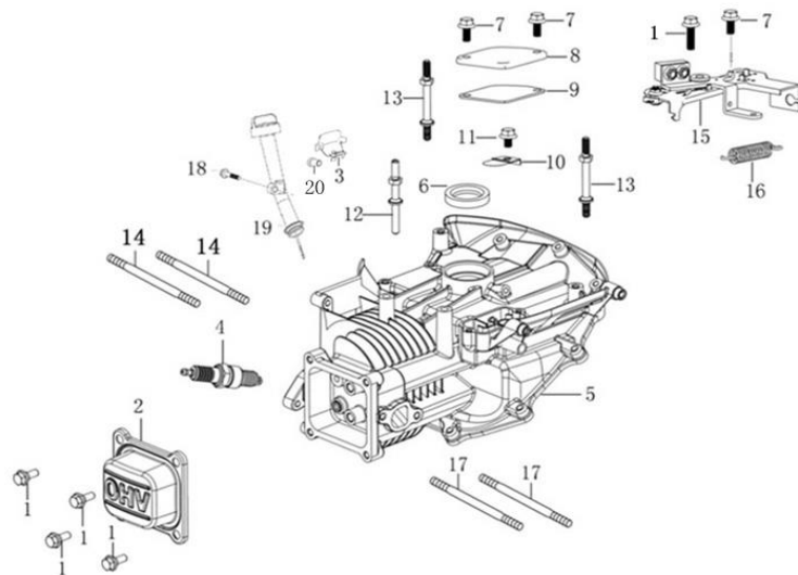
曲轴箱 (CRANK CASE)
