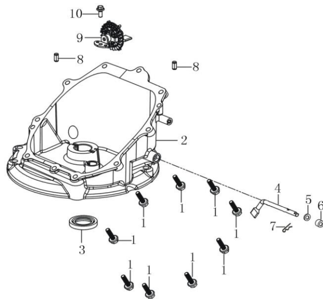
曲轴箱盖 (Crankcase cover)
