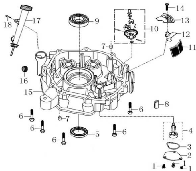
曲轴箱盖 (Crankshaft Cover)
