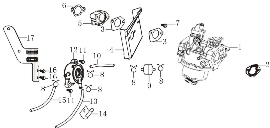
化油器 (Carburetor With Pump)
